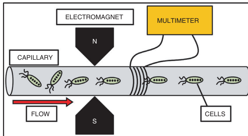
Figure 2 Diagrammatic representation of the experimental setup in which the voltage produced by different materials was tested. The suspensions were pumped from left to right in the capillary and magnetic materials were aligned by the electromagnet if it was needed. Materials then passed through the solenoid and induced an emf on the coil. This voltage was then measured by the multimeter and analysed. [Colour figure can be viewed at wileyonlinelibrary.com ]
